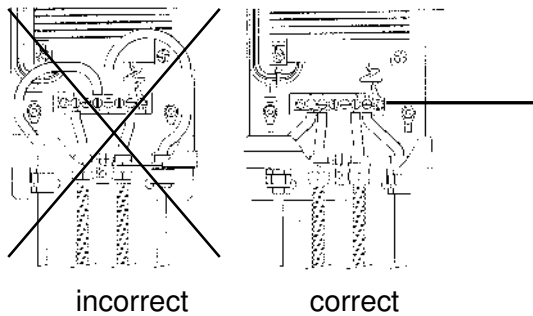
Figure 3: Cable connection in the power unit
